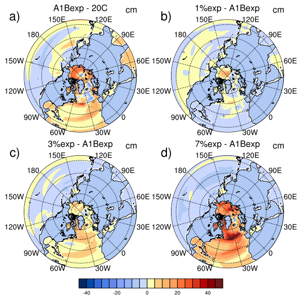
Figure 3. Dynamic sea level anomalies: (a) the mean of 2080–2099 in A1Bexp minus the mean of the last 20 year of the 20th century; (b–d) are the mean of 2080–2099 in 1%exp, 3%exp, and 7%exp minus the mean of 2080–2099 in A1Bexp, respectively.
