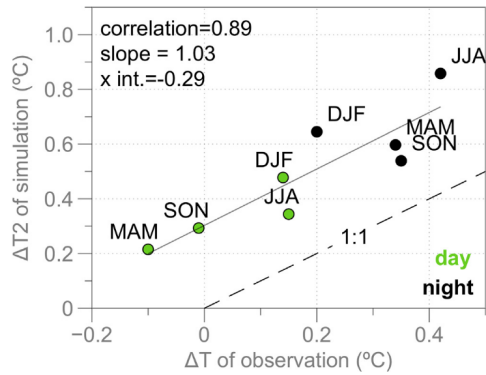
Figure 4. Comparison of Observations and Simulations for the Texas Location (Table 1) We compare day and night response over four seasons. Observations are surface (skin) temperature differences. Simulation is differences in 2-m air temperatures between the benchmark scenario (0.5 MW km -2 ) and control. Note that while correlation over eight points is high, the simulated response is larger, likely due to the much larger perturbed area and the difference between skin and 2 m air temperature.
